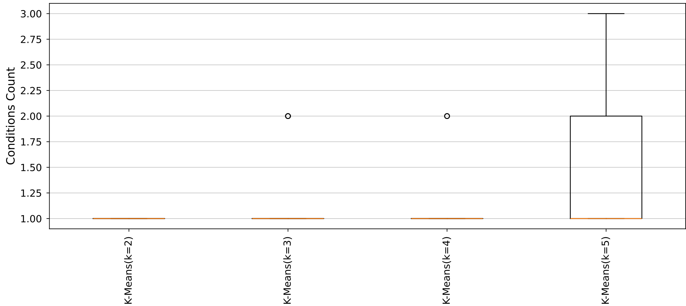
YARA Rules Conditions Count Distribution (Cluster43_Size5 dataset)
